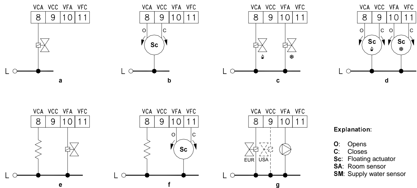
Fig. 7: Possible diagrams for valves connection.
